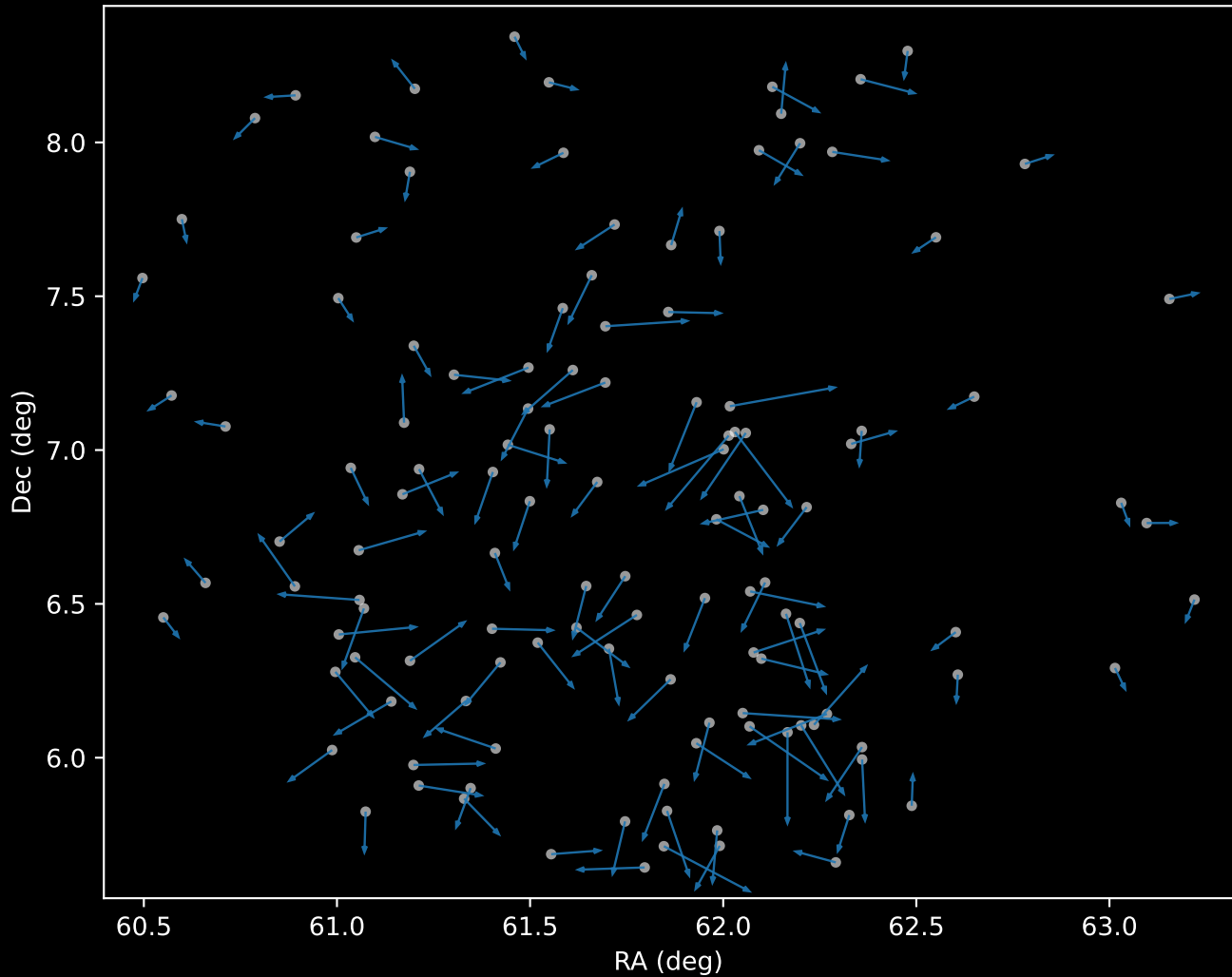
APOGEE DR17 Cluster 0 Proper Motion Vectors (n=123)
