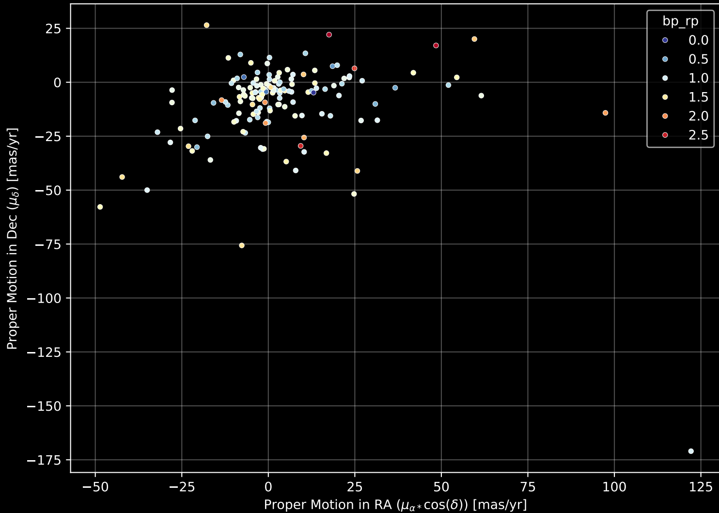
APOGEE DR17 Field: [060-30] Proper Motion Diagram (n= 154)
