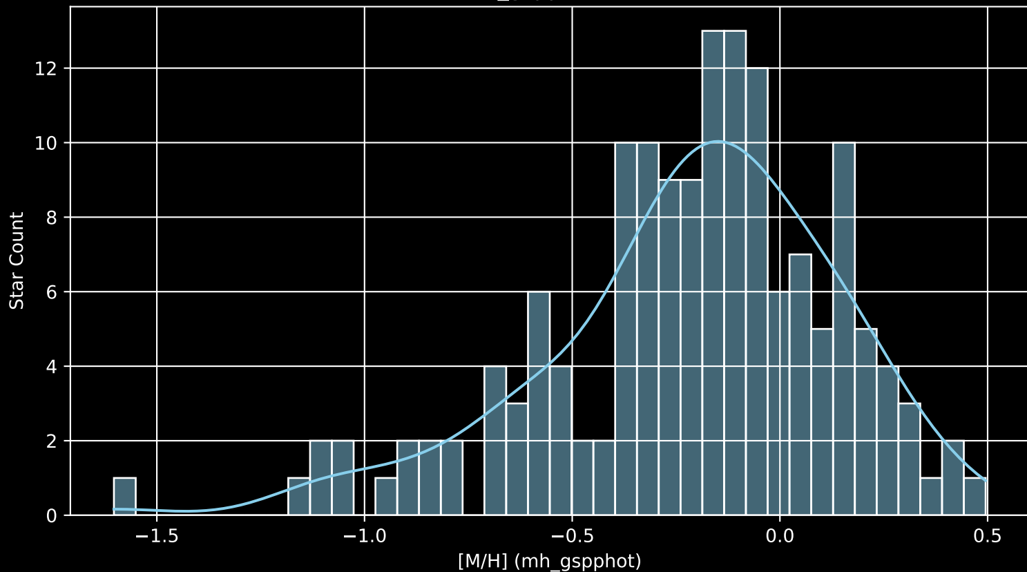
APOGEE DR17 Field: [060-30 [M/H] (mh_gspphot) (n= 154)
