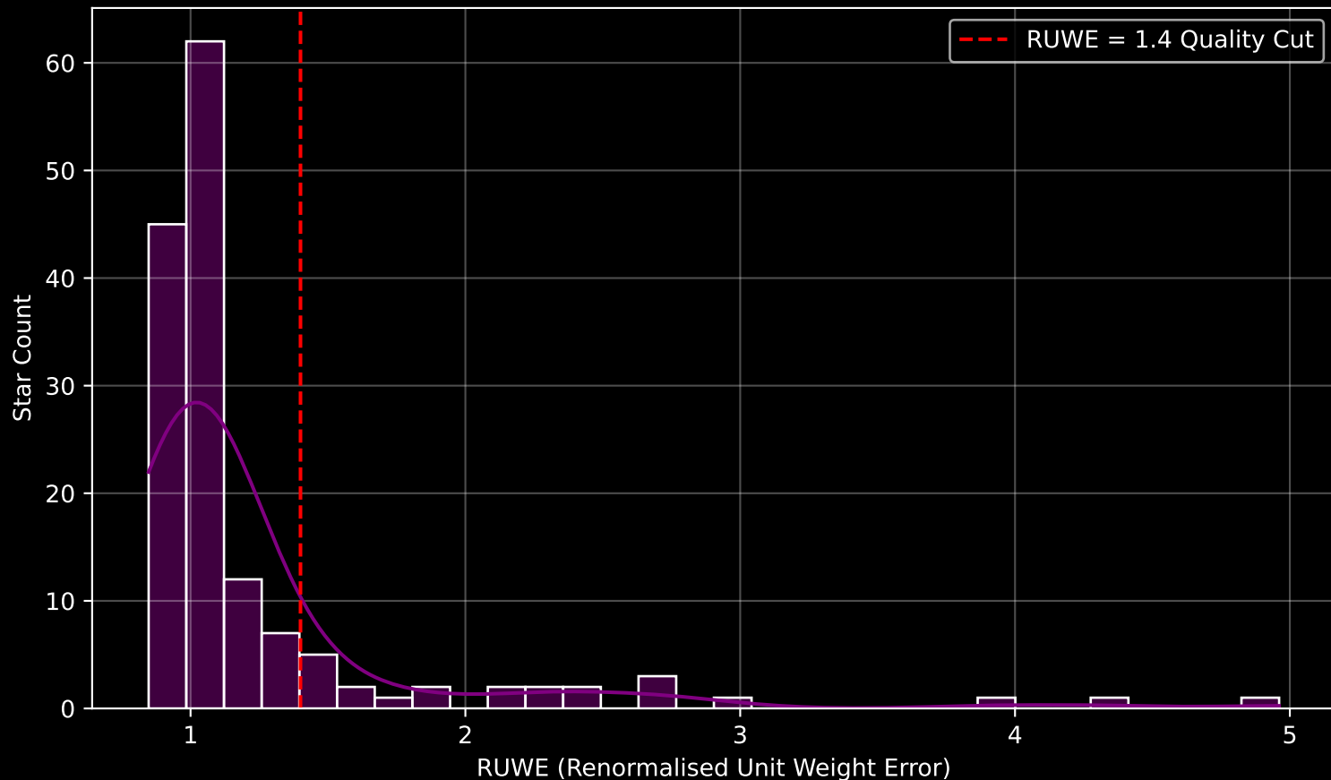
GAPOGEE DR17 Field [060-30] RUWE Distribution (n= 149)
