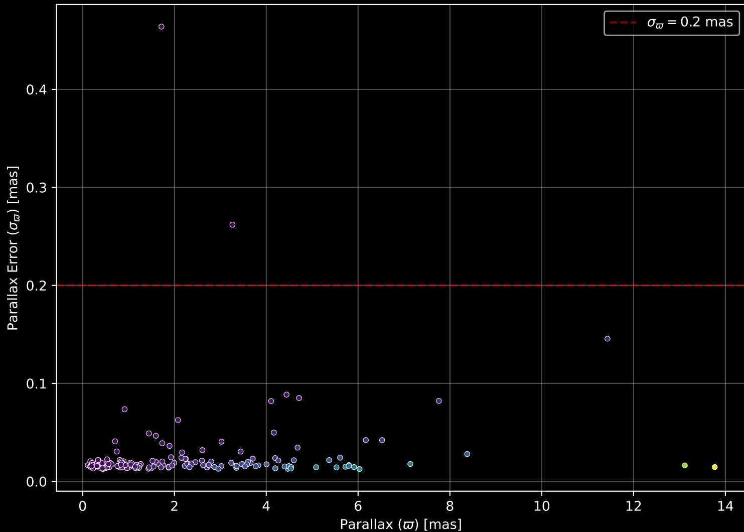
APOGEE DR17 Field: [060-30] Parallax Quality (n= 154)
