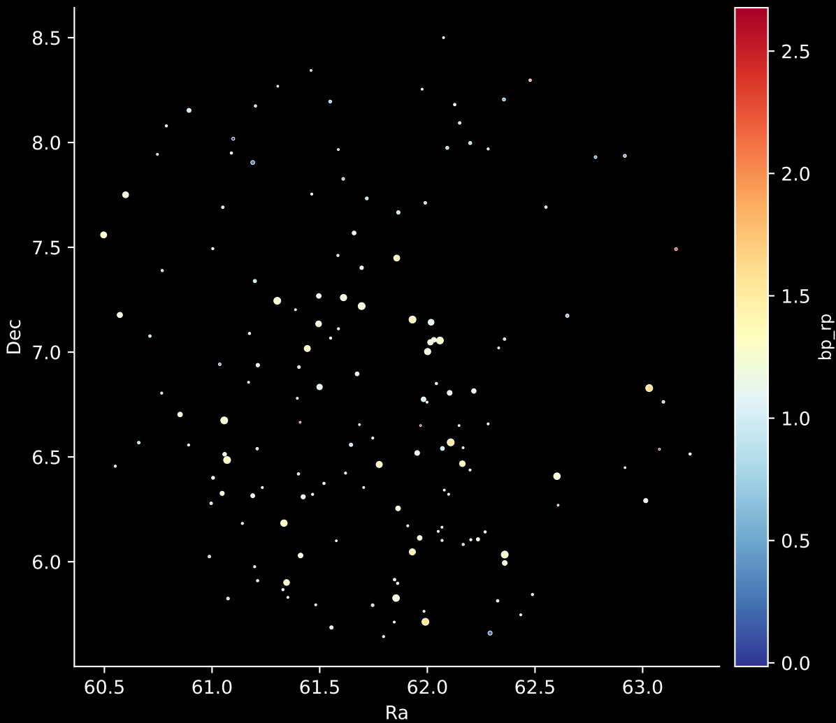
APOGEE DR17 Field: [060-30] Stars: 154
