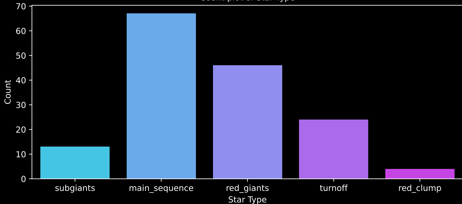
APOGEE DR17 Field: [060-30] Count plot of Star Type
